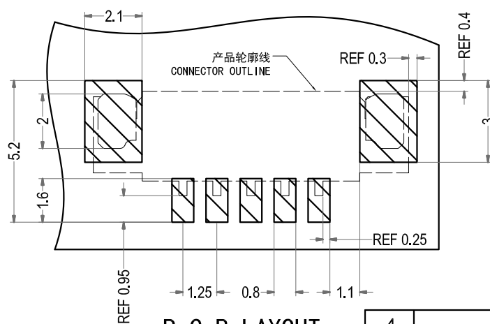
P. C. B LAYOUT
